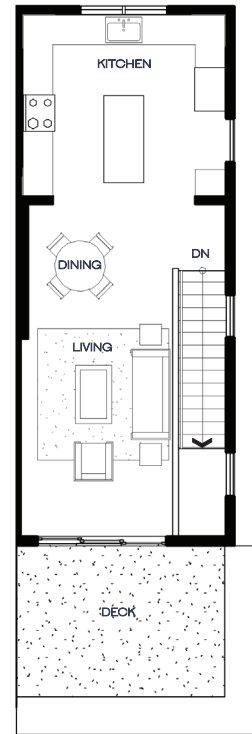
THIRD FLOOR
