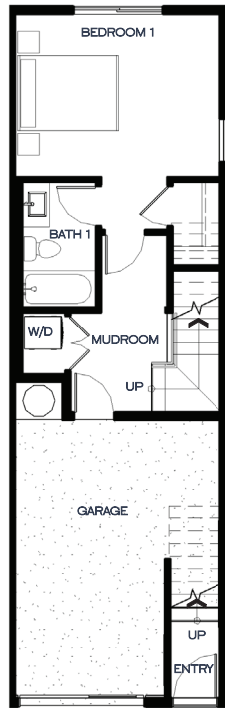
FIRST FLOOR
